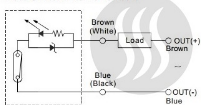
Auto Switch Internal Circuit
