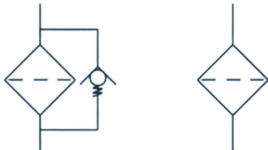
With By-pass Valve Without By-pass Valve
