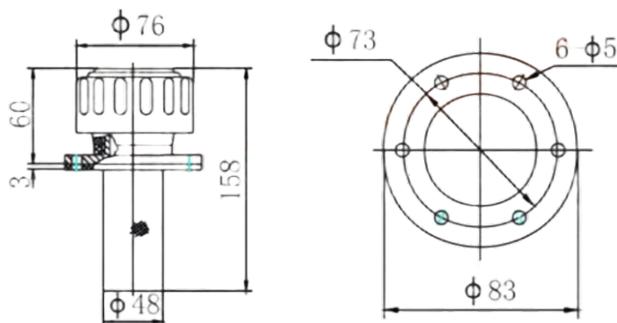
Flange Connection Type
